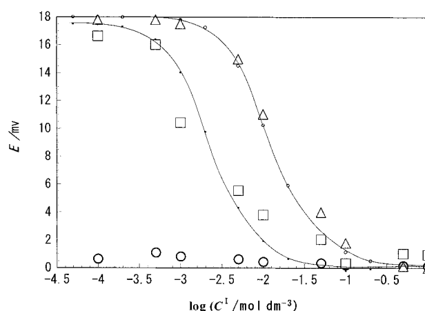
Fig. 6. Membrane Potential of PHEA, HA and HA-PHEA Gels □, HA-PHEA gel; △, HA gel; ○, PHEA gel. Solid curves are calculated values from Eq. 2 under C^I(\text{KCl})/C^{II}(\text{KCl})=2 .
