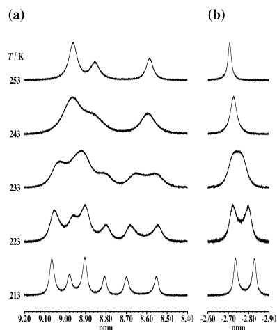
Fig. 5. ^1\text{H} -NMR Spectra for Compound 1' in \text{CDCl}_3 in the Range of 213 to 253 K
