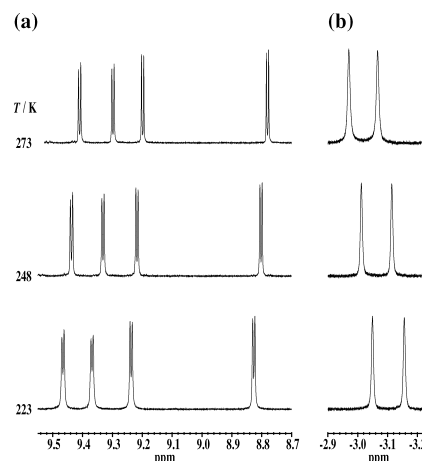
Fig. 4. ^1\text{H} -NMR Spectra for Compound 1 in \text{CDCl}_3 in the Range of 223 to 273 K
