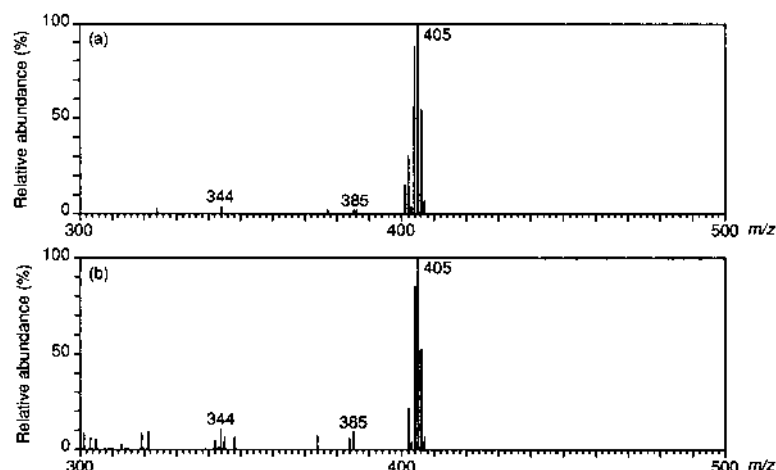
Fig. 10. APCI Mass Spectra of Alkaloids Recorded by Solvent System of 0.05 M Ammonium Acetate in D_2O -Acetonitrile-Tetrahydrofuran
