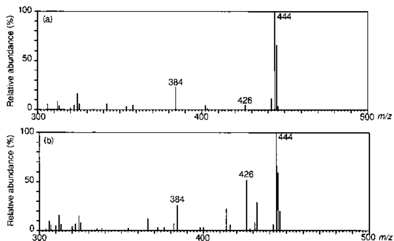
Fig. 2. APCI Mass Spectra of Alkaloids 12,15-Diacetyluciculine ( 1 ; a) and 12,15-Diacetyl-1- epi -luciculine ( 2 ; b)
