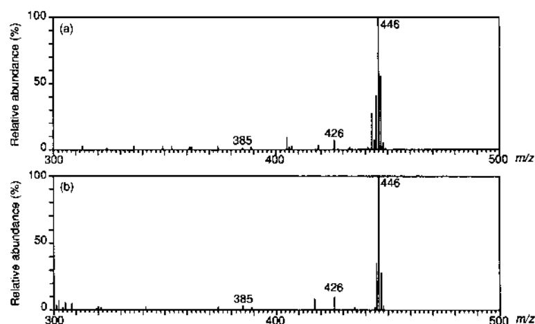
Fig. 5. APCI Mass Spectra of Alkaloids Recorded by Solvent System of 0.05 M Ammonium Acetate in D_2O -Acetonitrile-Tetrahydrofuran (a) 12,15-Diacetyl-luciculine (1), (b) 12,15-diacetyl-1- epi -luciculine (2). The drift voltage between the first and the second electrodes was 140 V.
