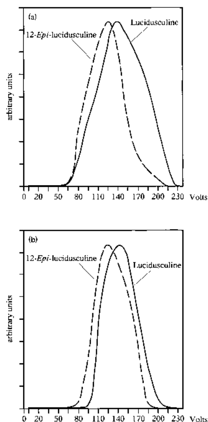
Fig. 9. Ion Currents of the Fragment Ions at m/z 384 (a) and m/z 342 (b) Arising from Alkaloids Lucidusculine ( 5 , Solid Line) and 12- Epi -lucidusculine ( 6 , Dashed Line) as a Function of the Drift Voltage between the First and the Second Electrodes of the APCI Ion Source
