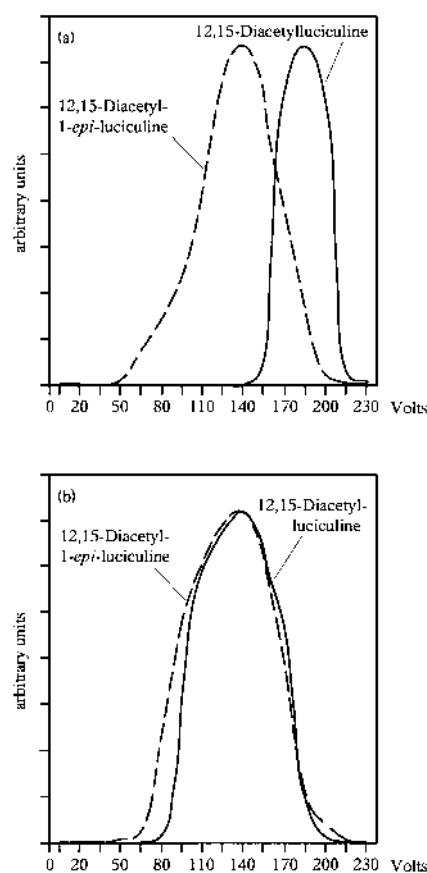
Fig. 4. Ion Currents of the Fragment Ions at m/z 426 (a) and m/z 384 (b) Arising from Alkaloids 12,15-Diacetyluciculine (1, Solid Line) and 12,15-Diacetyl-1- epi -luciculine (2, Dashed Line) as a Function of the Drift Voltage between the First and the Second Electrodes of the APCI Ion Source
