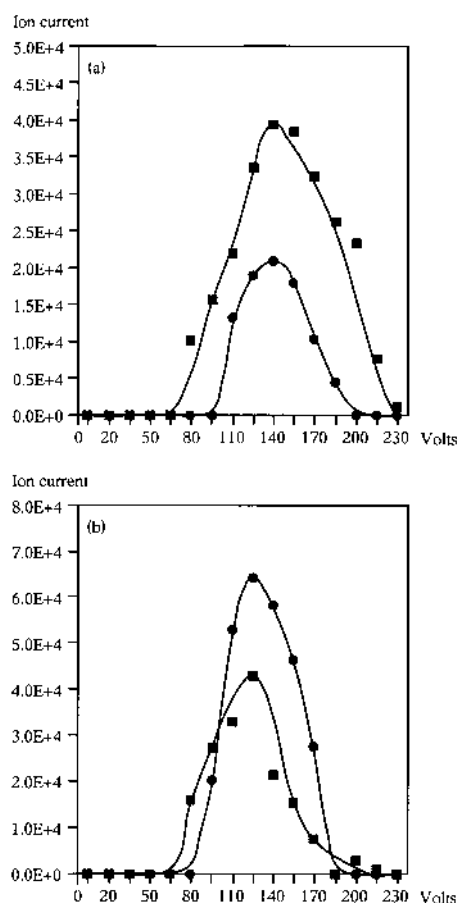
Fig. 8. Ion Currents of the Fragment Ions at m/z 384 (■) and m/z 342 (●) Arising from Alkaloids Lucidusculine ( 5 ; a) and 12- Epi -lucidusculine ( 6 ; b) as a Function of the Drift Voltage between the First and the Second Electrodes of the APCI Ion Source
