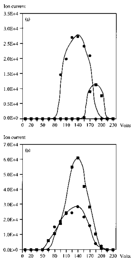
Fig. 3. Ion Currents of the Fragment Ions at m/z 426 (■) and m/z 384 (●) Arising from Alkaloids 12,15-Diacetyluciculine (1; a) and 12,15-Diacetyl-1- epi -luciculine (2; b) as a Function of the Drift Voltage between the First and the Second Electrodes of the APCI Ion Source
