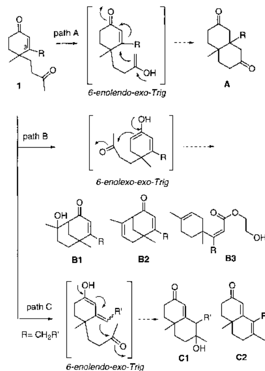
Chart 2. Possible Reaction Path from 1
