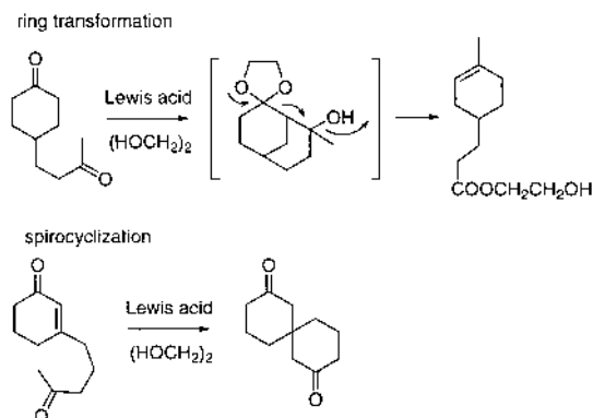
Chart 1. Reactions Using a Combination of Lewis Acid and 1,2-Diol
