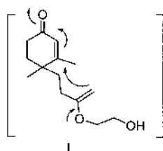
Fig. 1. Plausible Intermediate for Path A
