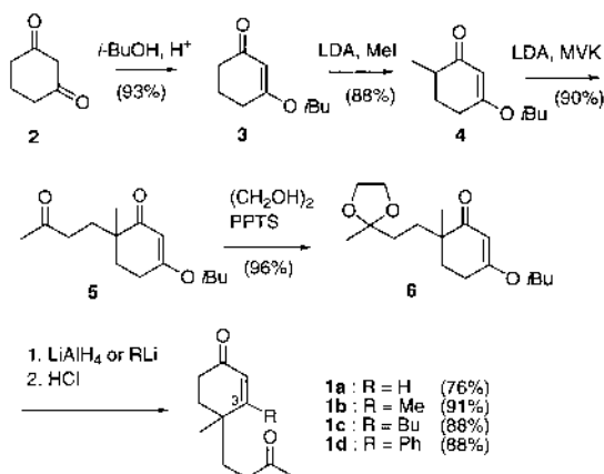
Chart 3. Preparation of Substrates 1a–d
