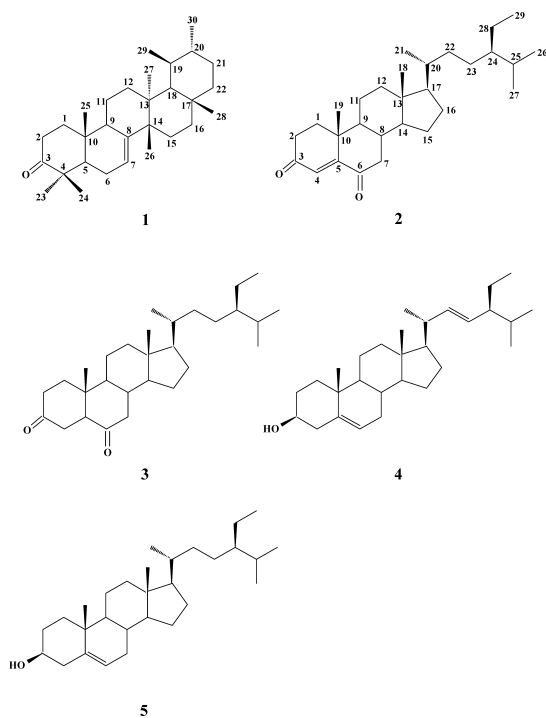
Fig. 2. Chemical Structures of the Isolated Components from Gleditsia sinensis
