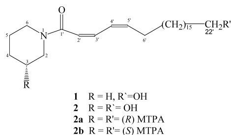
Fig. 1. Structures of Haloxyline A ( 1 ) and Haloxyline B ( 2 )
